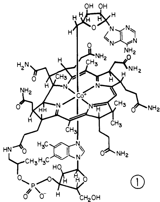
Figure 1. The vitamin B 12 coenzyme.
